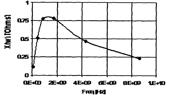
Fig. 3. Calculated X(\omega) for network of Fig. 1. with f_0=1.5\text{GHz} , R_m=4\text{Ohm} and R_f=0.48\text{Ohm}
