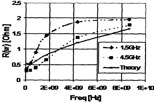
Fig. 2. Calculated R(\omega) for network of Fig. 1. R_m=4\text{Ohm} and R_f=0.48\text{Ohm} and different f_0
